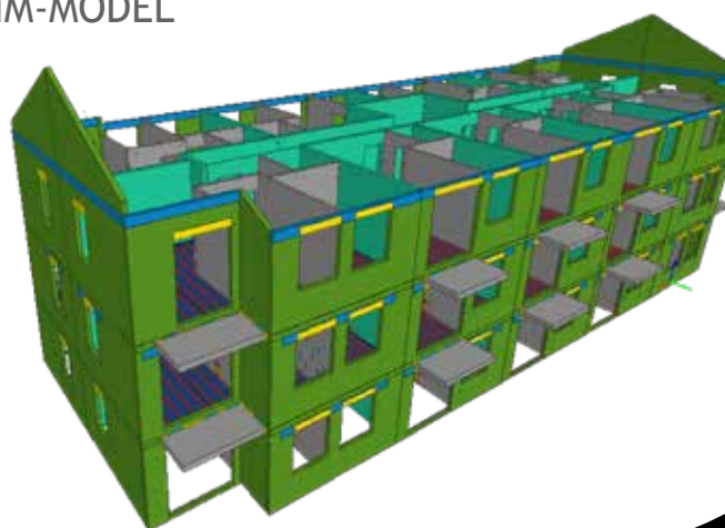
BIM-MODEL
